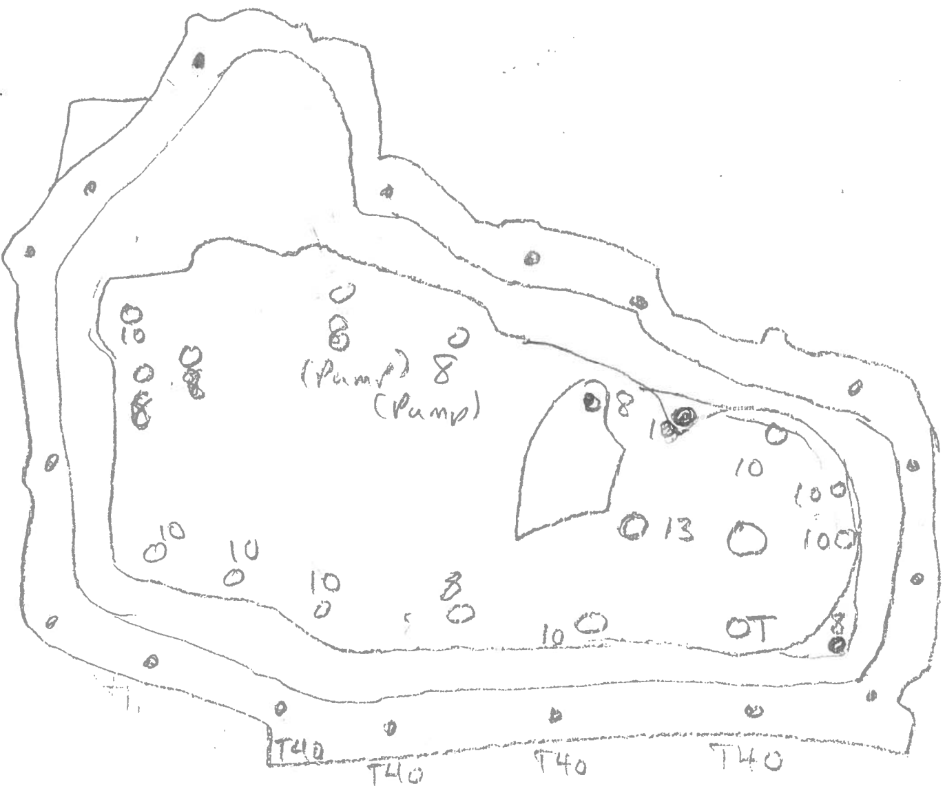
Channel plate bolt arrangements.
